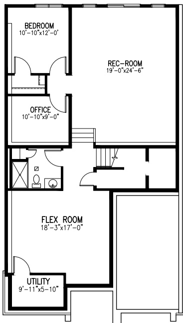
LOWER FLOOR = 1490 SQ.FT.
