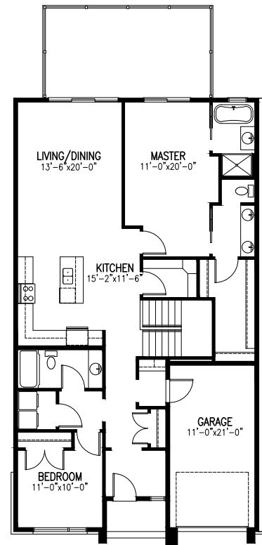
MAIN FLOOR = 1490 SQ.FT. GARAGE = 271 SQ.FT.
